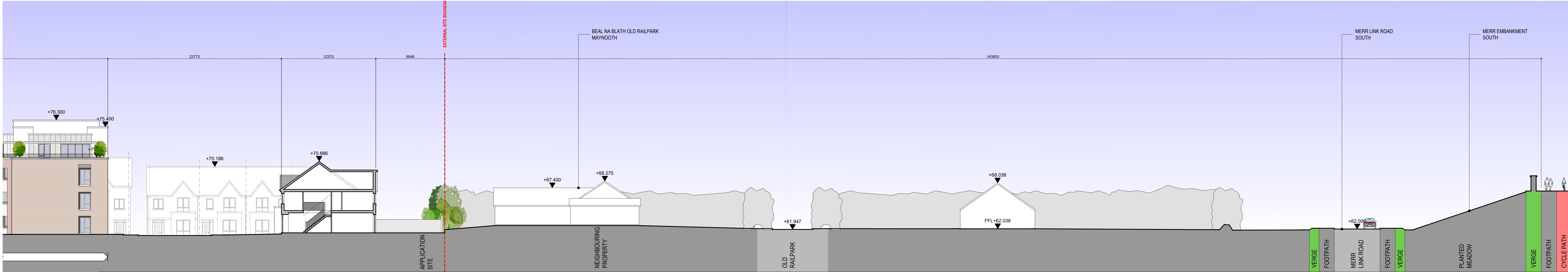
MEER CONTEXT ELEVATION 5-5 Scale 1:200
